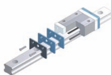
Figure 5.4 Sealing option GG
